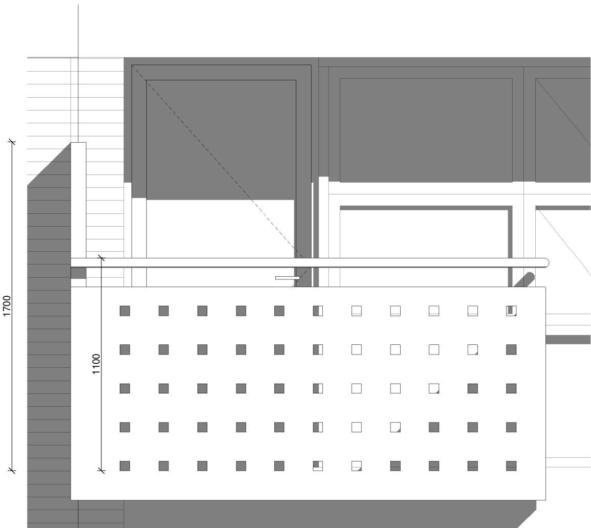
Elevation altan lille B | 1 : 20
