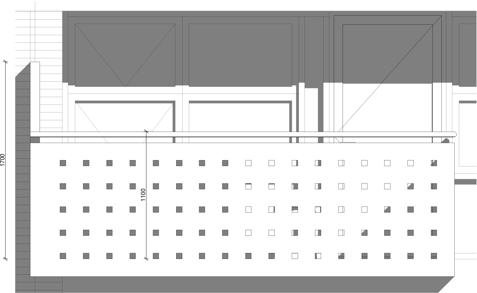
Elevation altan stor D | 1 : 20
